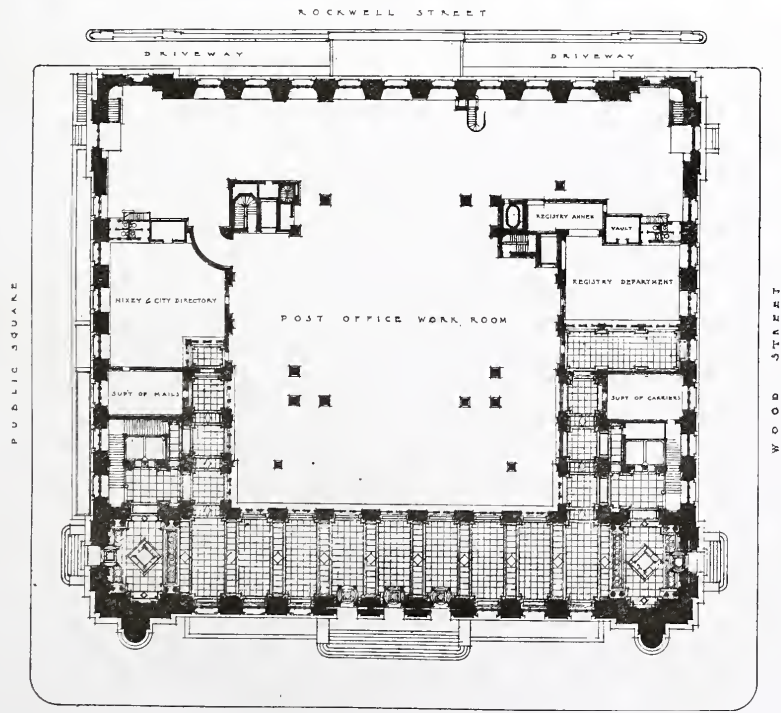
FIRST FLOOR PLAN (POST OFFICE).
